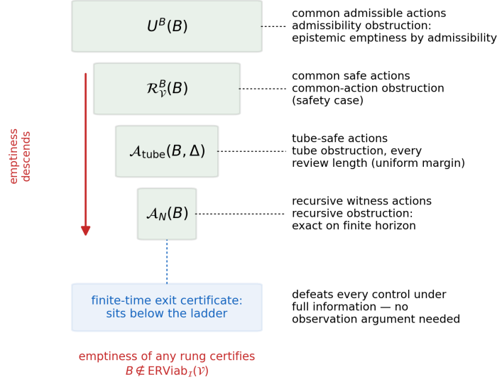
Figure 1: The obstruction ladder. The common response sets form nested necessary conditions for viability, U^B(B) \supseteq \mathcal{R}_V^B(B) \supseteq \mathcal{A}_{\text{tube}}(B, \Delta) \supseteq \mathcal{A}_N(B) , and emptiness descends (Proposition 2); the finite-time exit certificate sits below the ladder, defeating every control under full information (Theorem 4).
